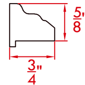
MOULDING B
