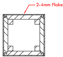
Profile E-E
